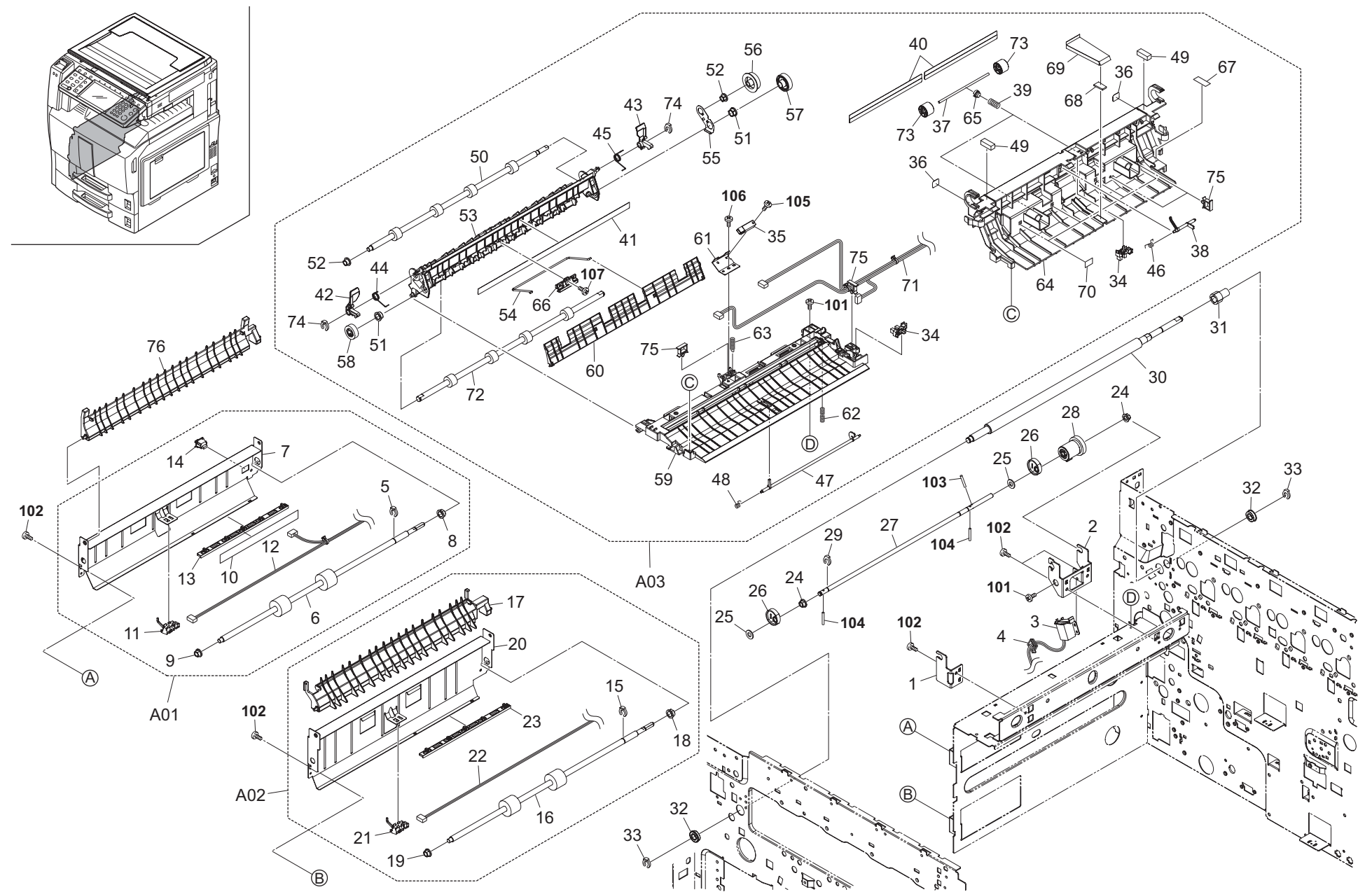
FIG. 12 Paper Conveying Section 1 (25/25, 30/30 ppm)
