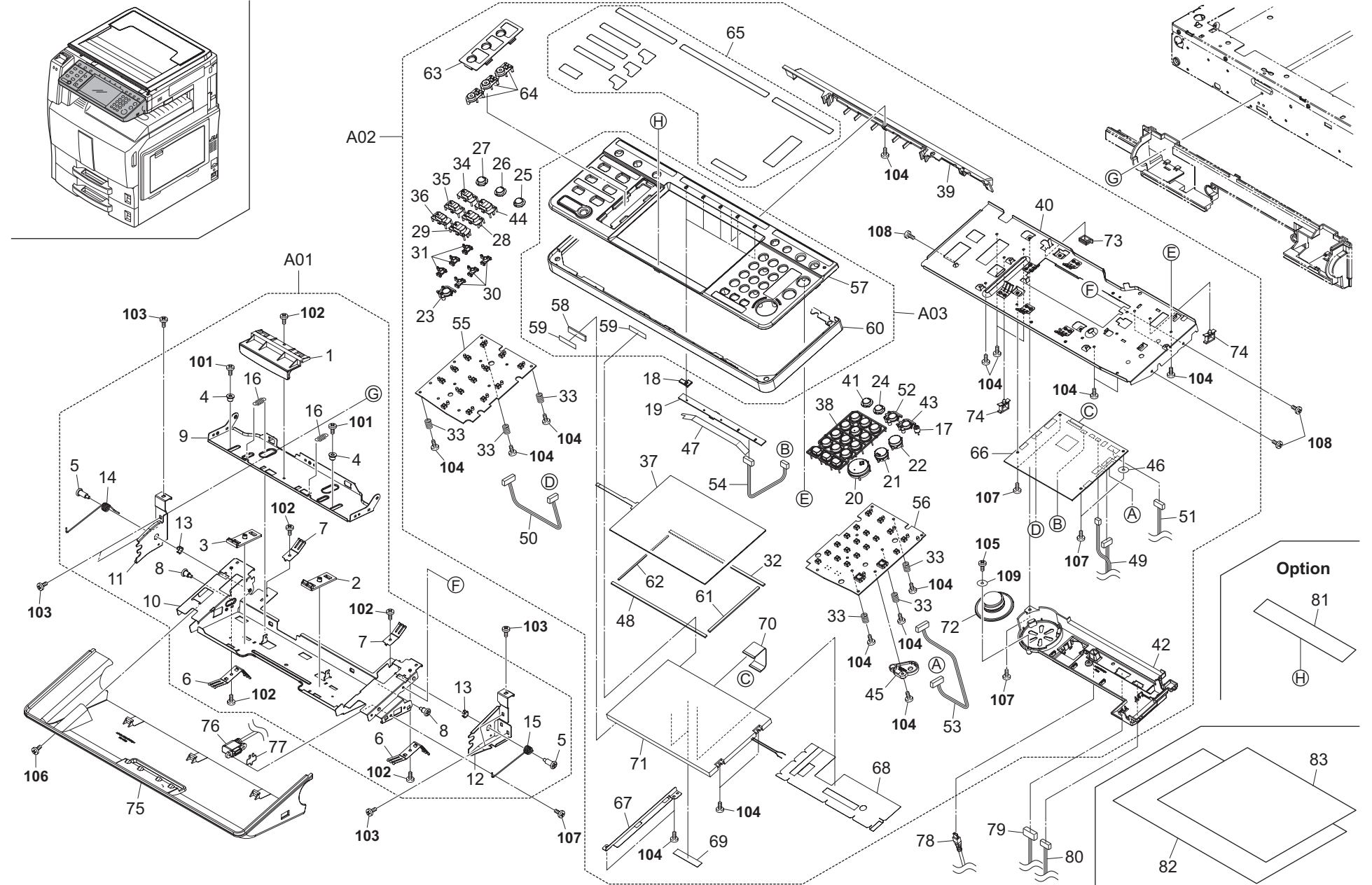
FIG. 30 Operation Section
