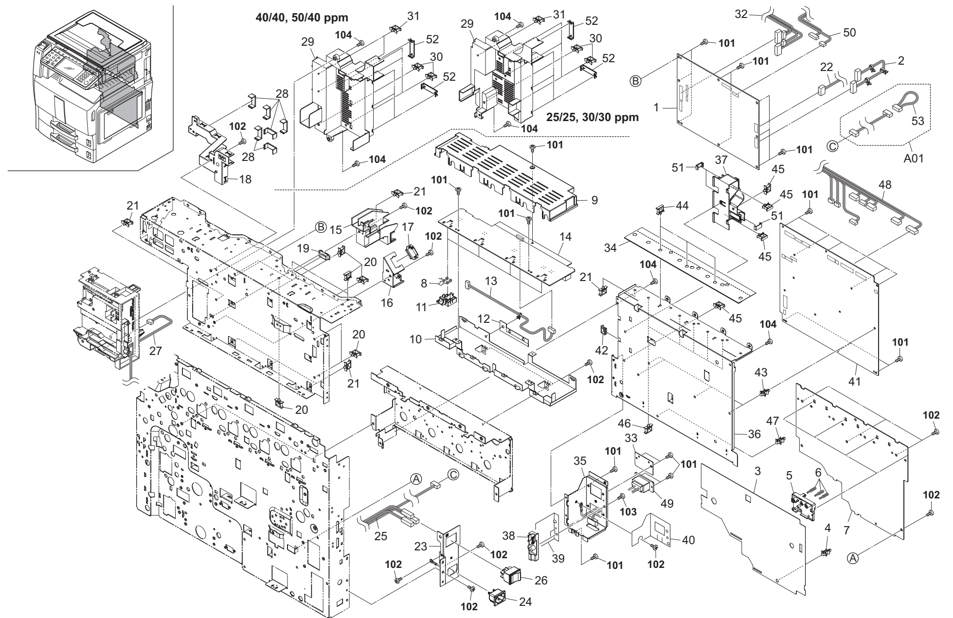
FIG. 28 Electrical Components 2
