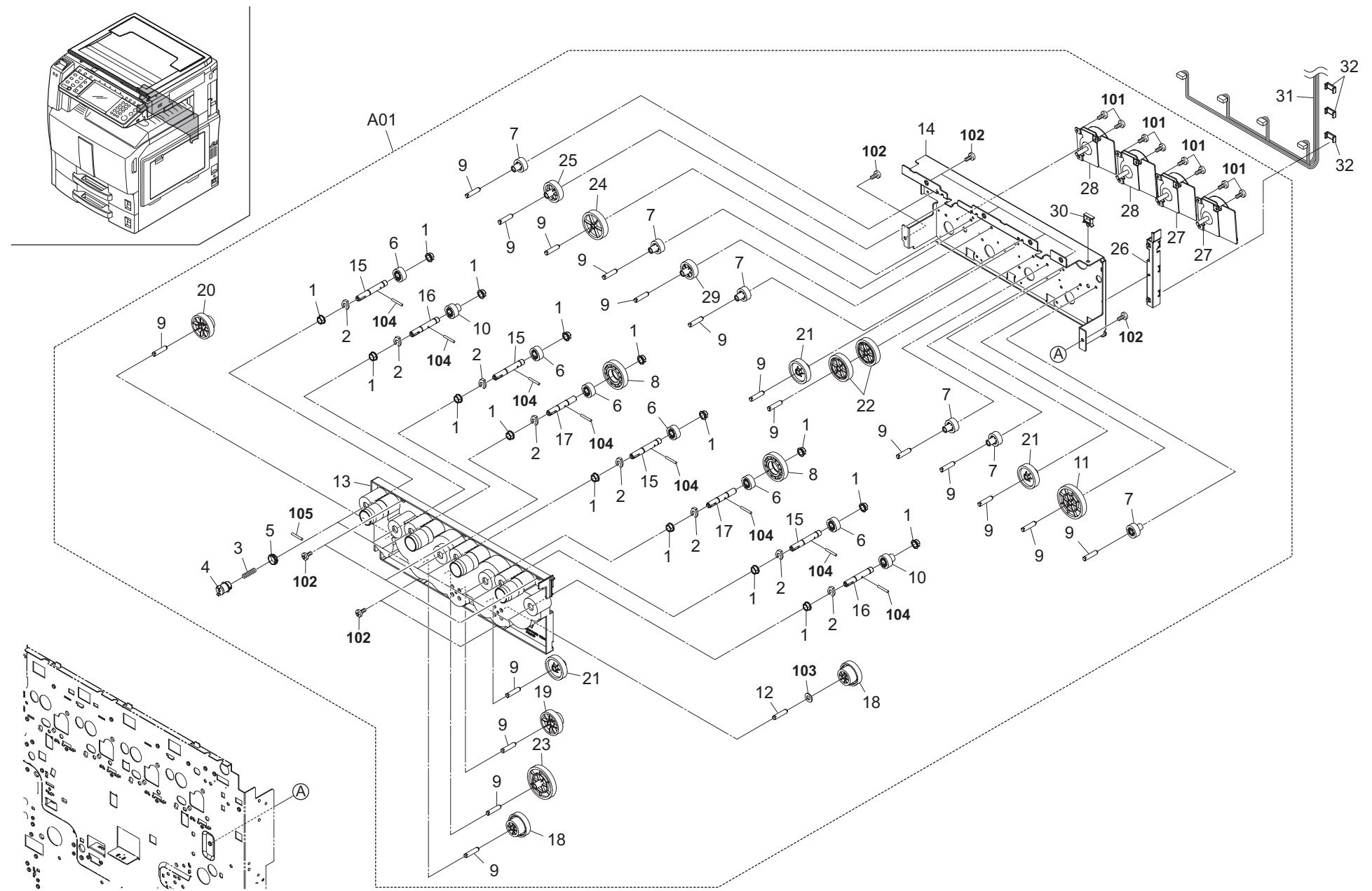
FIG. 20 Drive Section 1 (40/40, 50/40 ppm)
