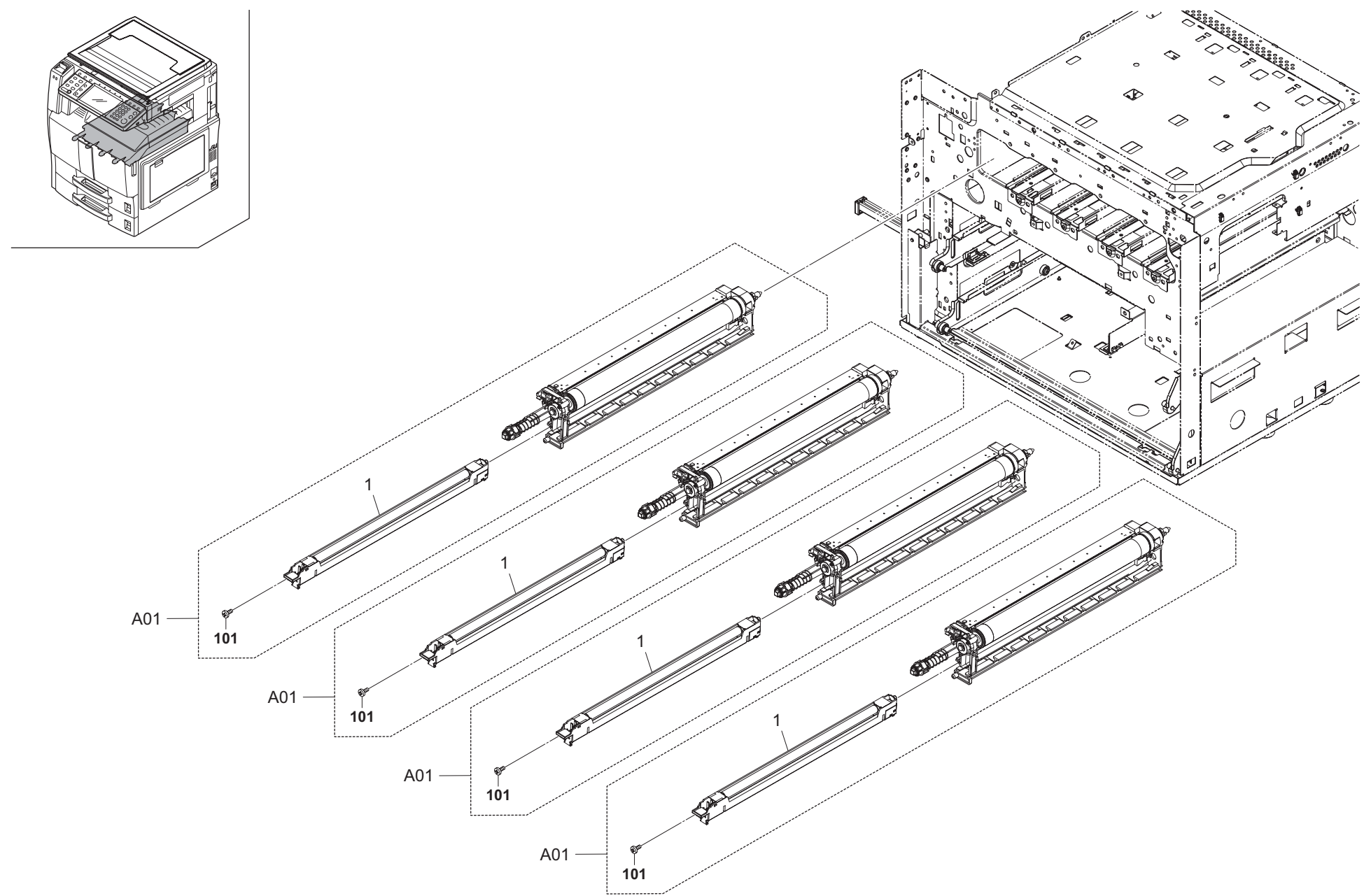
FIG. 17 Image Formation Section
