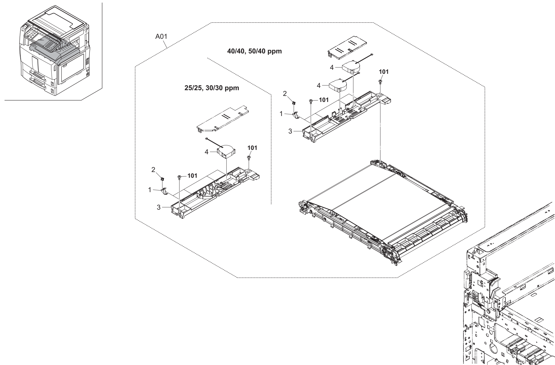
FIG. 11 Transfer Section
