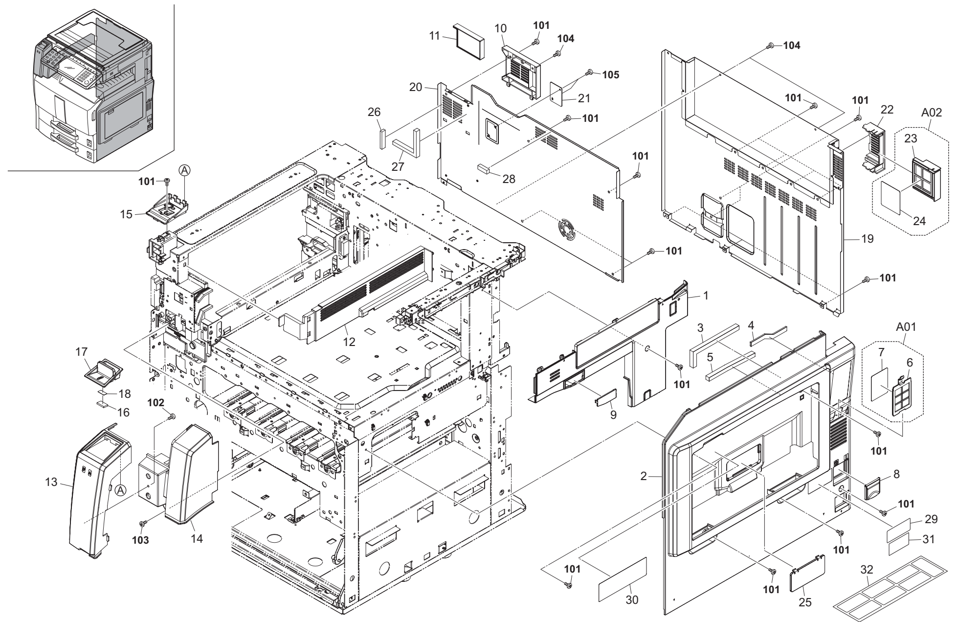
FIG. 2 Covers 2
