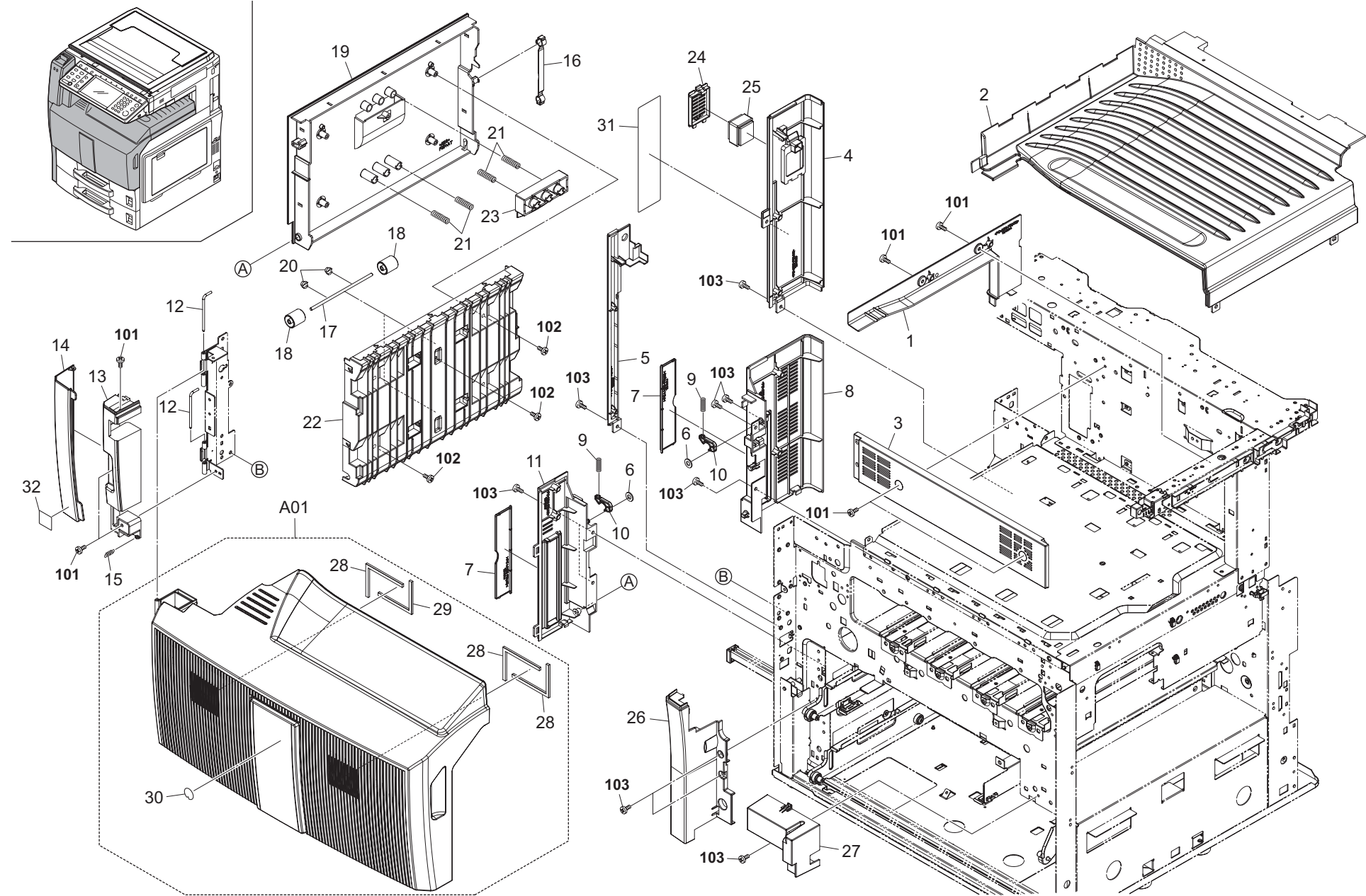
FIG. 1 Covers 1
