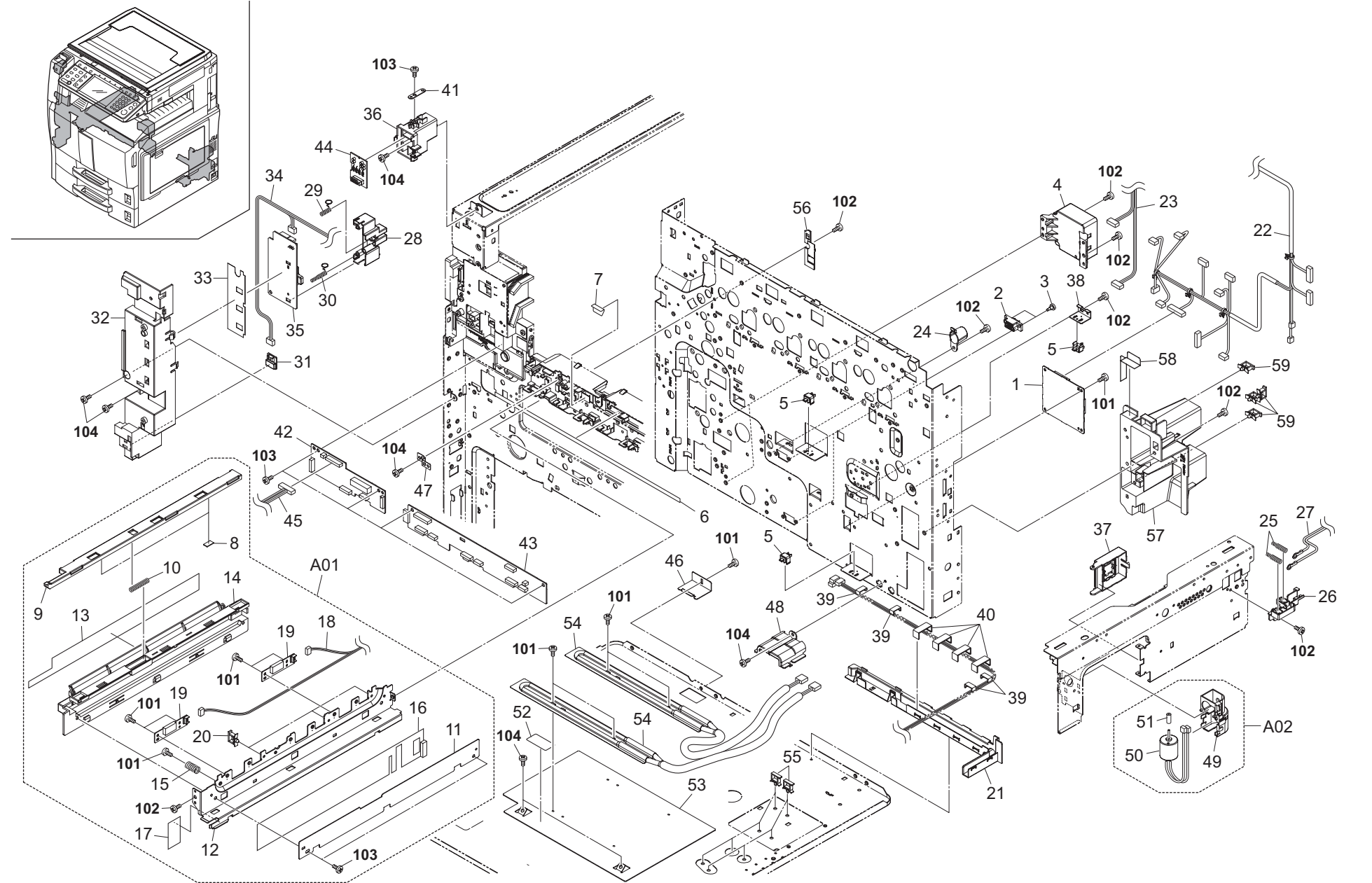
FIG. 27 Electrical Components 1
