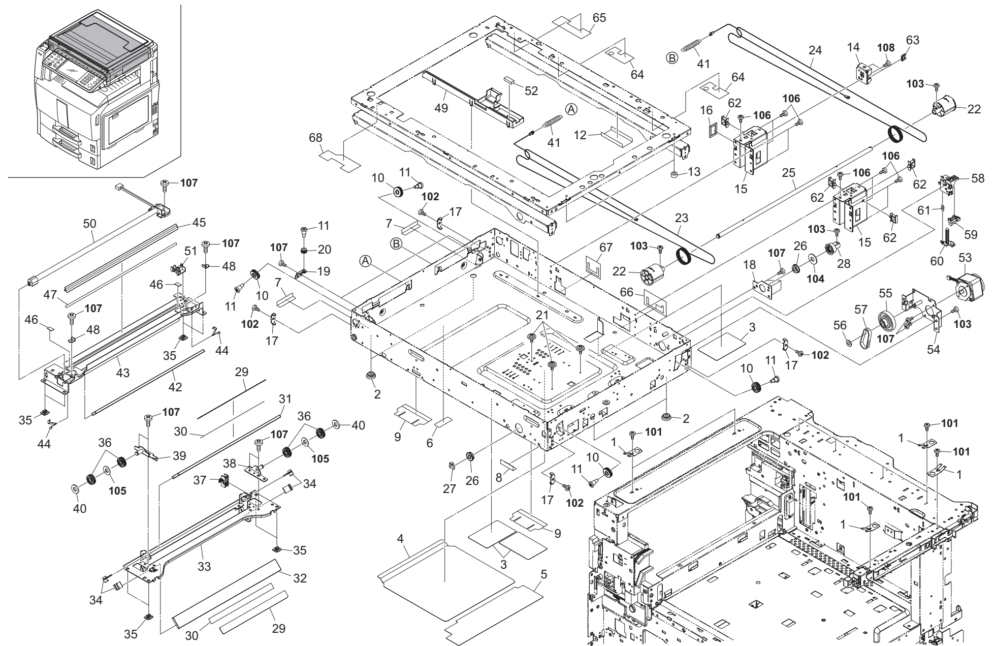
FIG. 14 Scanner Section 1
