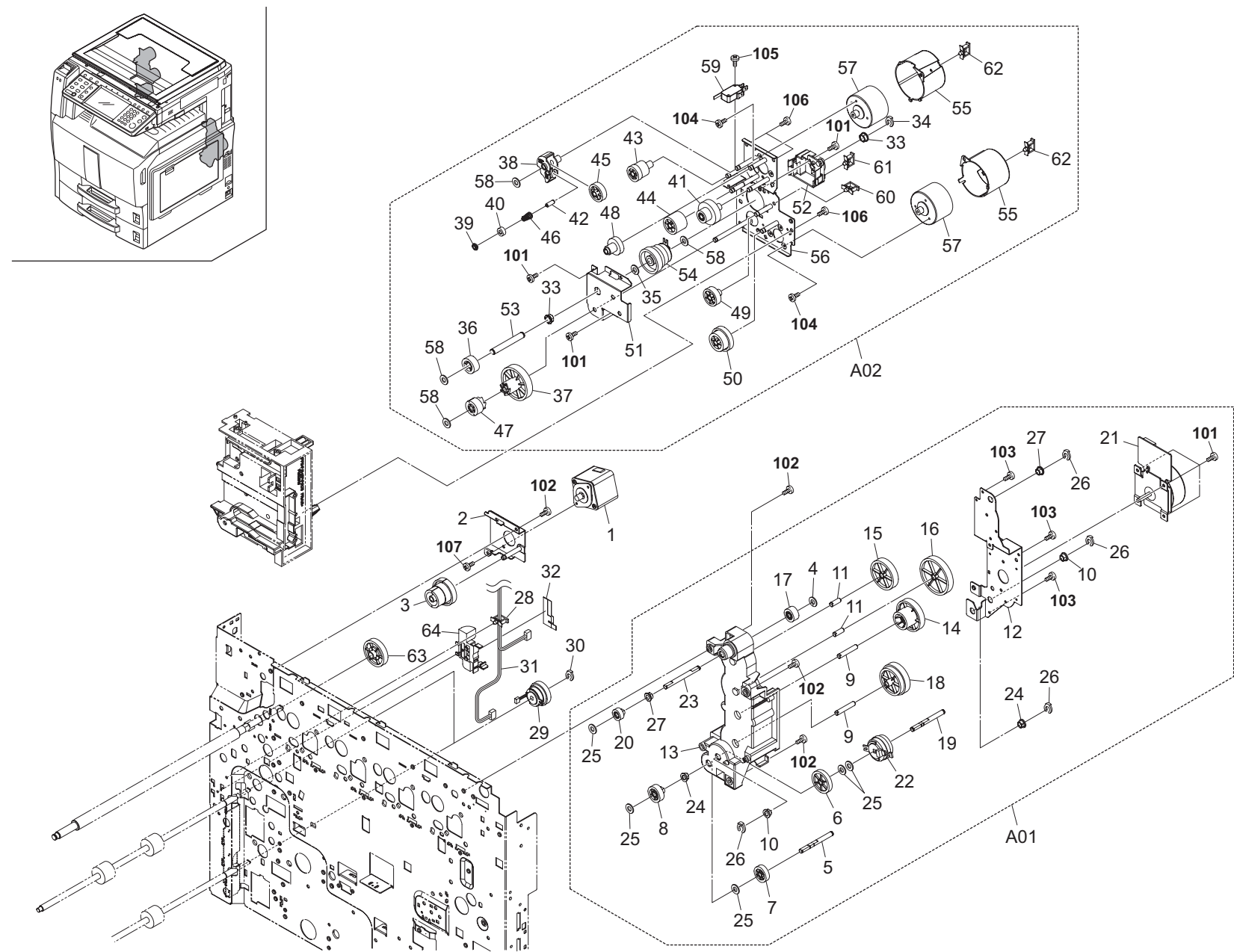
FIG. 21 Drive Section 2 (40/40, 50/40 ppm)
