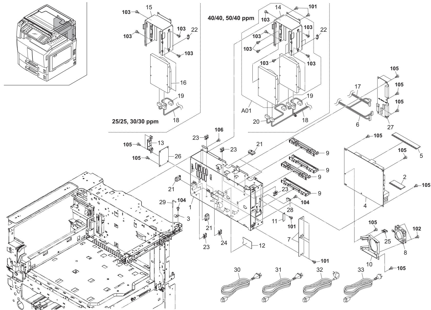
FIG. 29 Electrical Components 3
