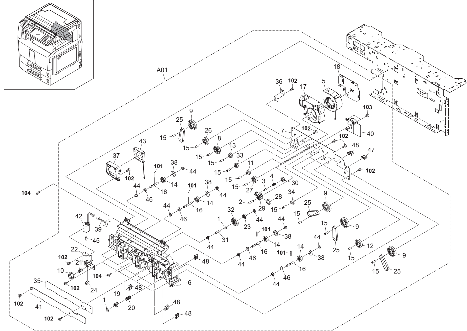
FIG. 23 Drive Section 4
