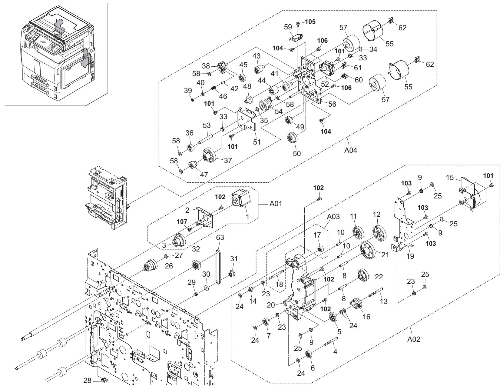
FIG. 21 Drive Section 2 (25/25, 30/30 ppm)
